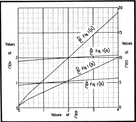
Fig. 4. Economic proportions for components carrying polarizing d.c.
