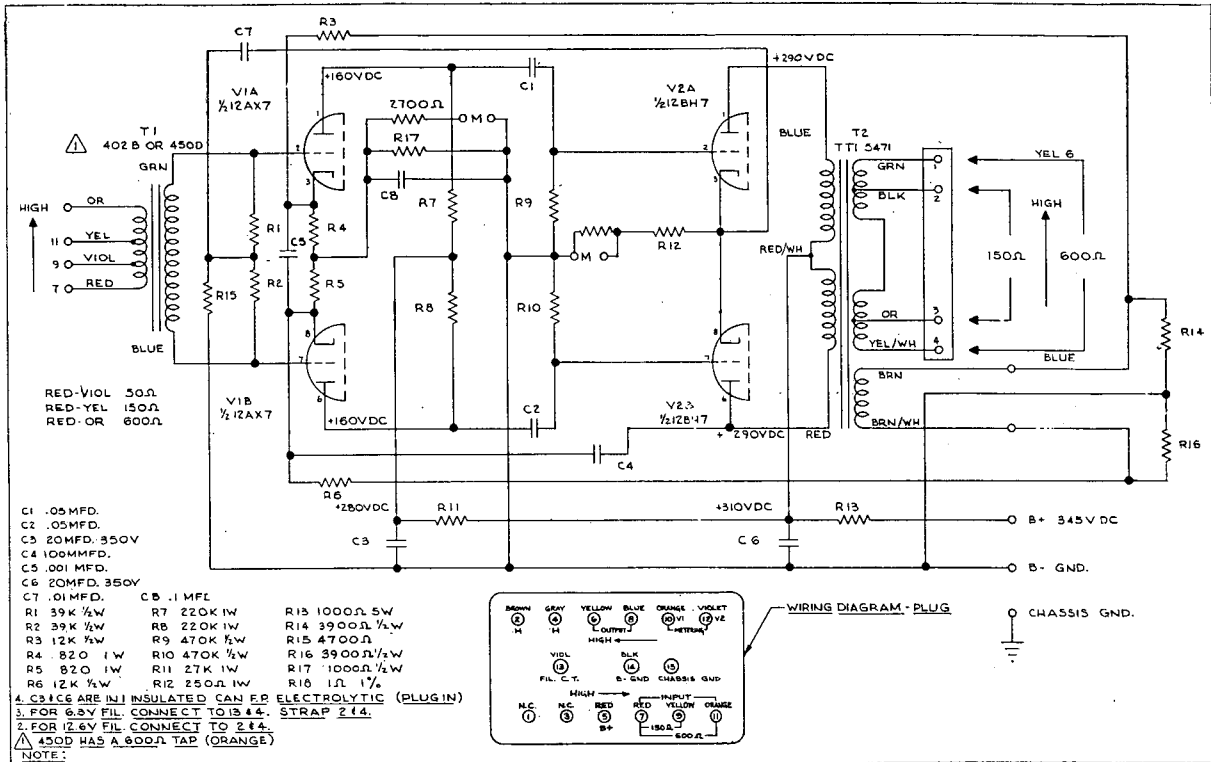
FIG. 11. Schematic of Model 101D program amplifier.
