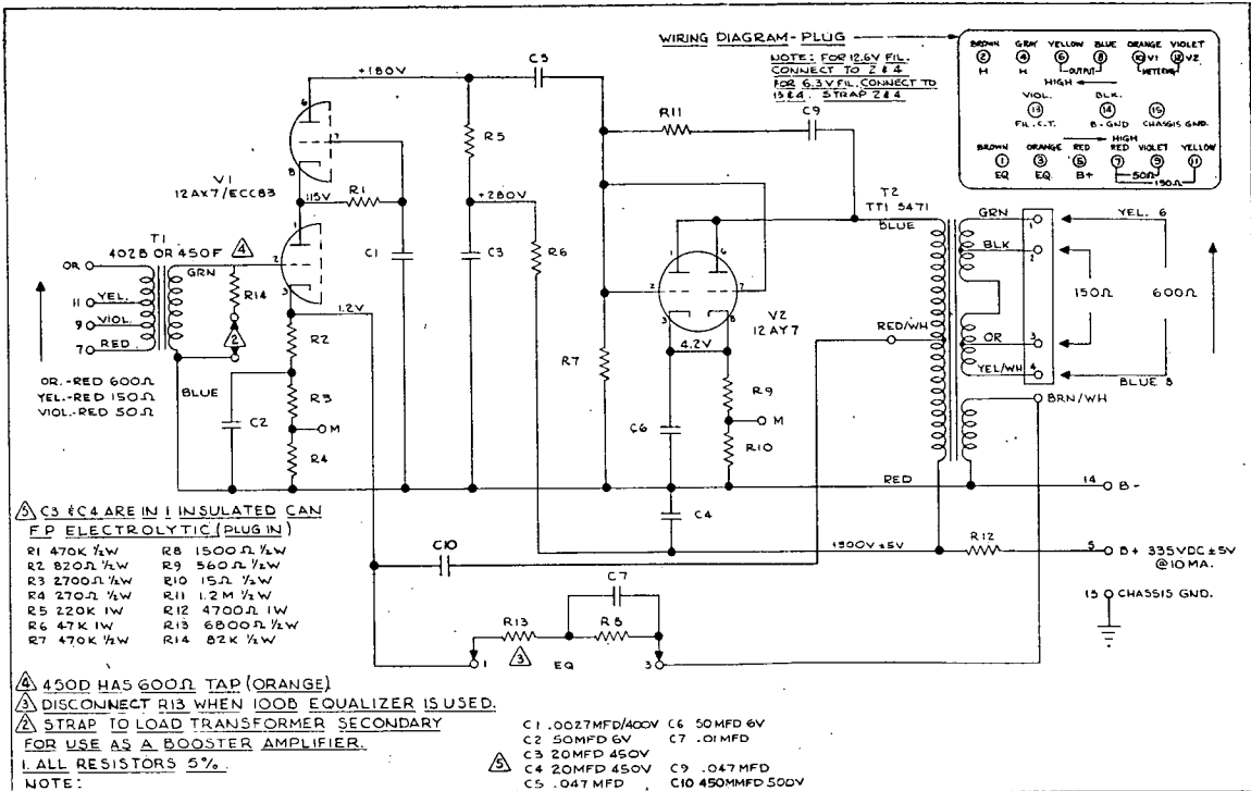
FIG. 8. Schematic of Model 100D microphone preamplifier.
