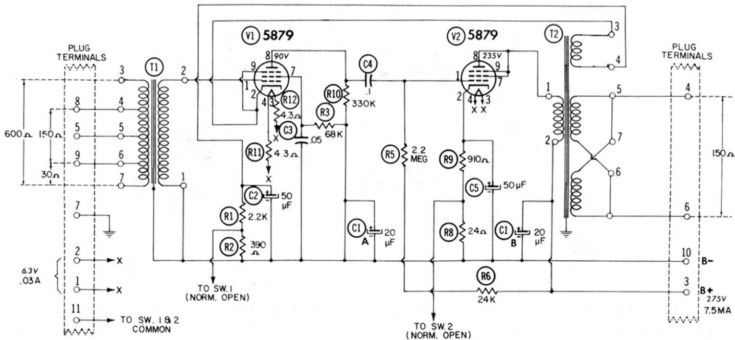
Fig. 12-85F. Circuit diagram of Langevin type 5116 plug-in amplifiers.
